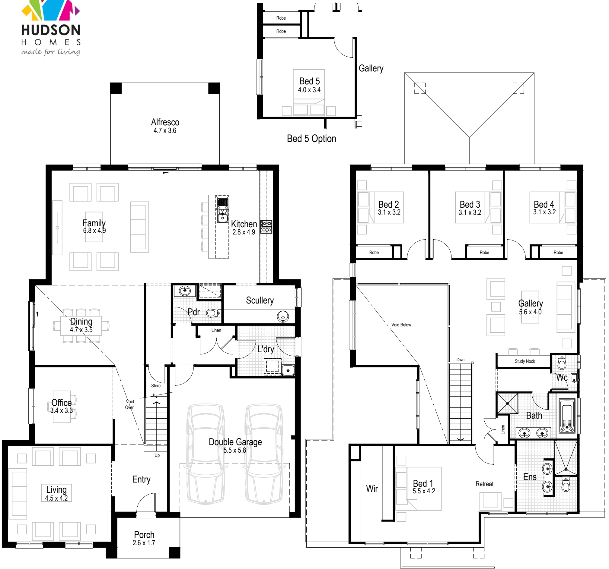
Ground Floor
